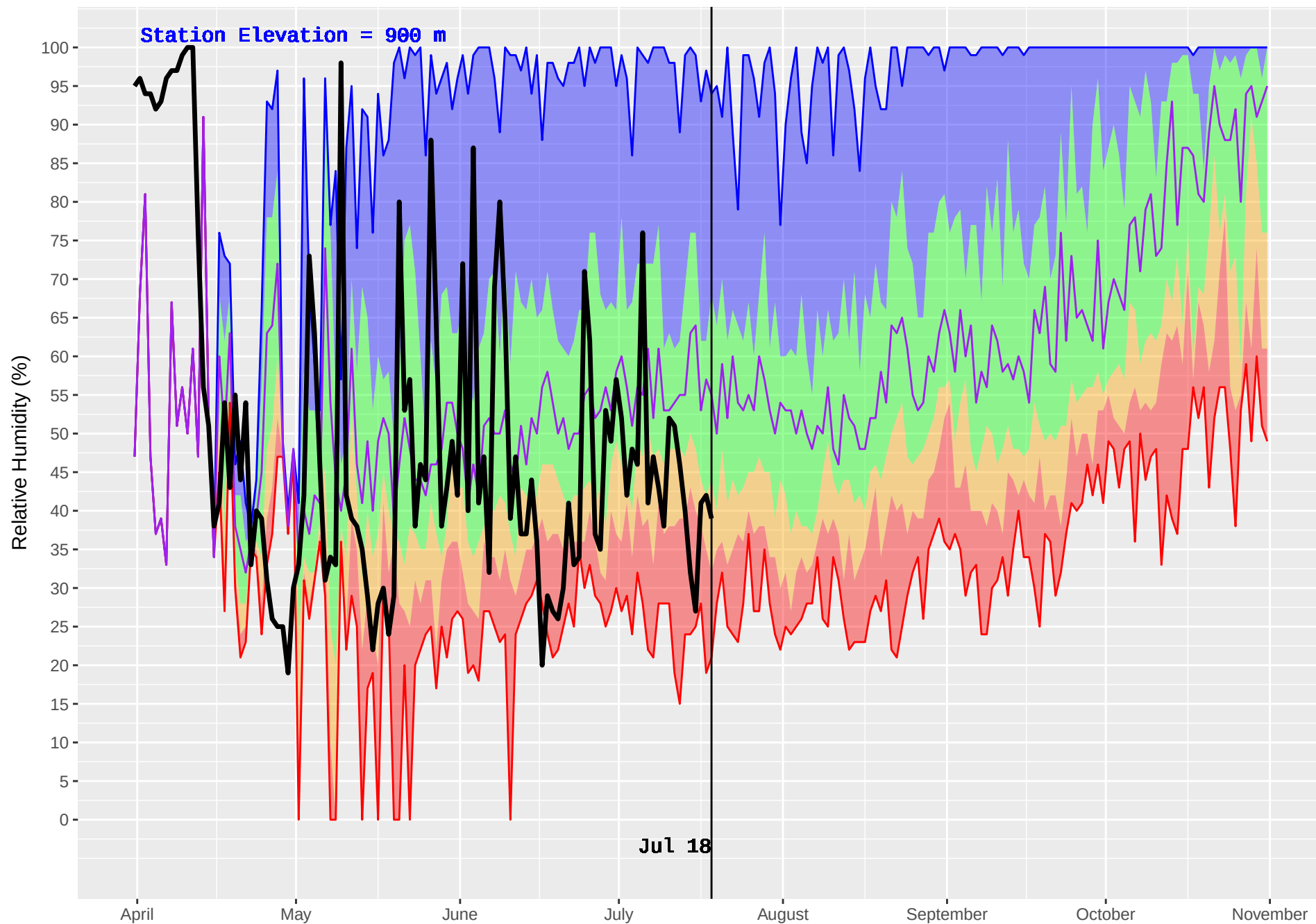
UPPER FULTON (169) : Historical (1986–2016) and Current (2018) Daily Relative Humidity
